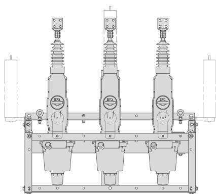
Viper-ST recloser
