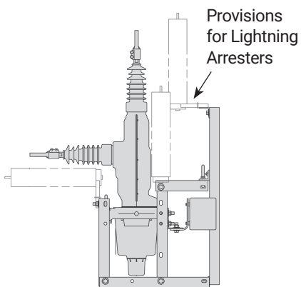
Viper-ST recloser
