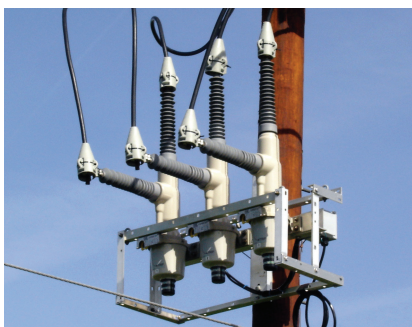
Center polemount Viper ® -ST recloser
