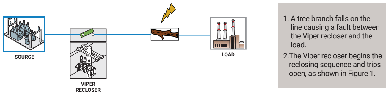
Figure 1: Stand-alone Viper recloser trips on a fault
