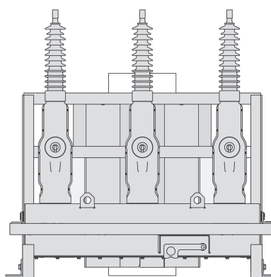
Viper-S recloser
