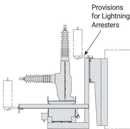
Viper-S recloser
