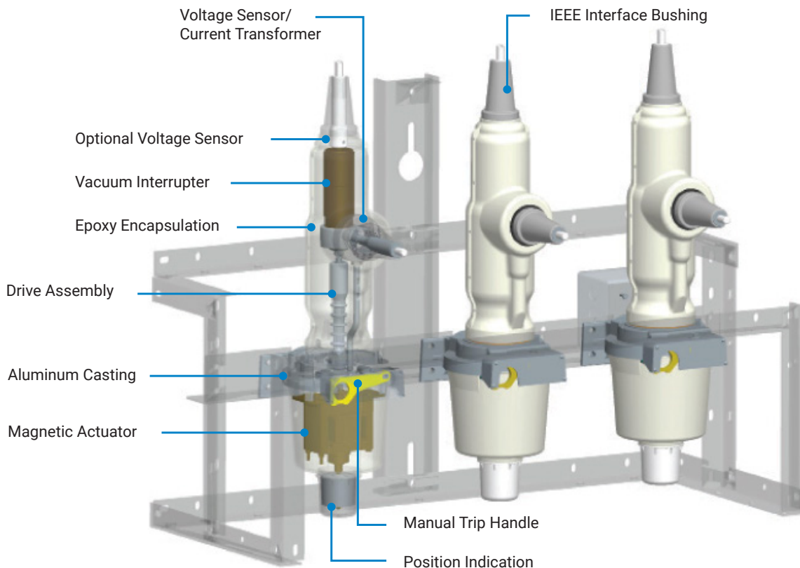
Isometric view of the Viper-ST without insulators.
