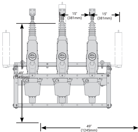
38kV center polemount Viper-ST
