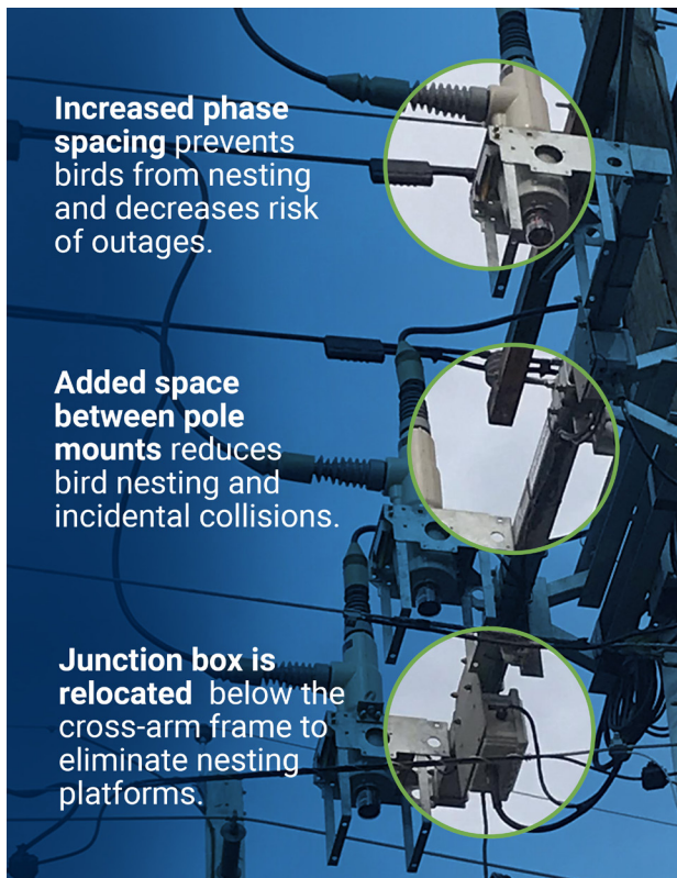
Viper®-ST Crossarm Design
